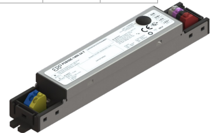
Terminal Blocks: "-T" Suffix L 154.2 x W 26.2 x H 21.85 mm (L 6.07 x W 1.03 x H 0.86 in.)
